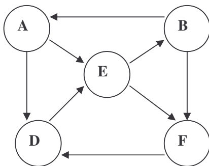
Fig 1: Co-citing
