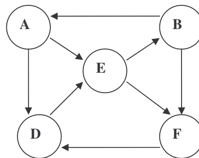
Fig 2: Colinking
